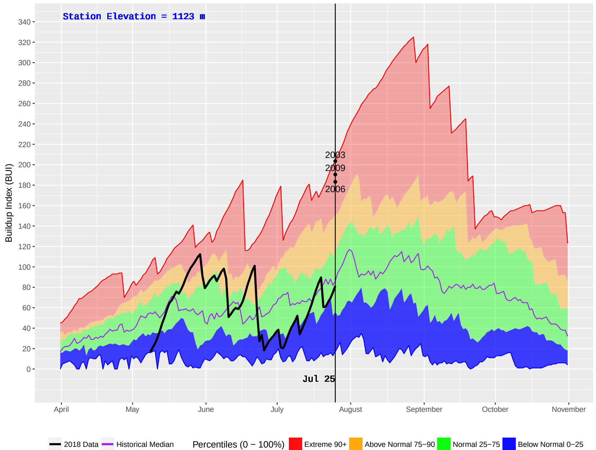
MCLEAN LAKE (311) : Historical (1987–2016) and Current (2018) Noon Buildup Index (BUI)
