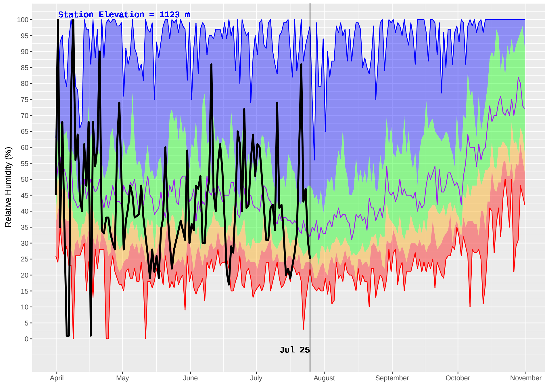
MCLEAN LAKE (311) : Historical (1987–2016) and Current (2018) Noon Relative Humidity
